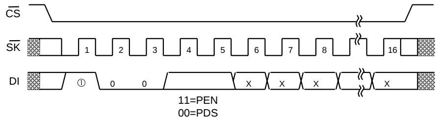
Figure 9 PEN/PDS Timing
