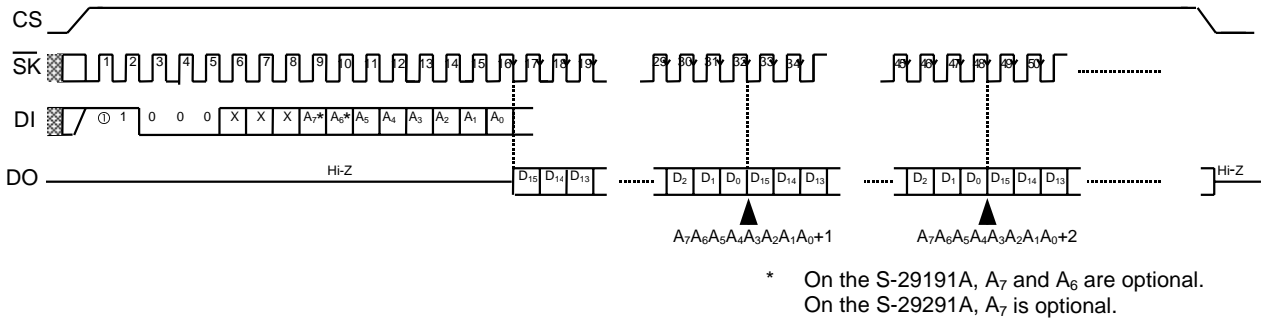
Figure 5 Read Timing (S-29391A)
