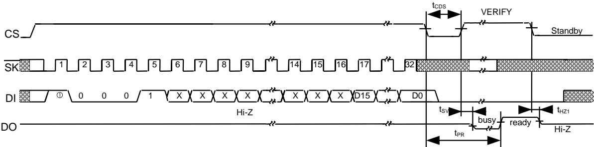
Figure 7 WRAL Timing
