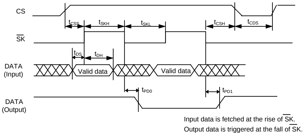
Figure 3 Timing chart
