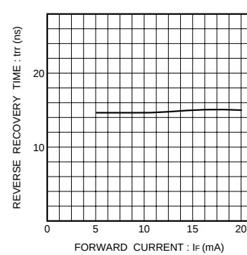
Fig. 6 Reverse recovery time characteristics
