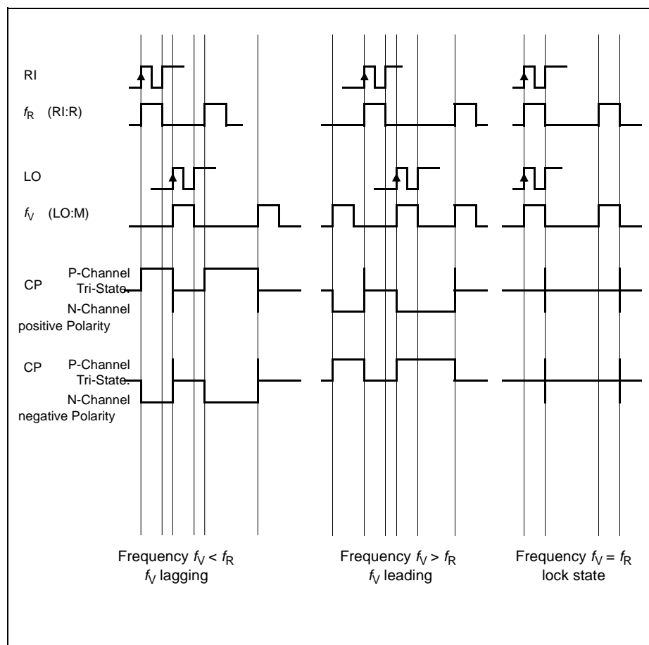
Figure 3-3 Frequency detector output waveforms
