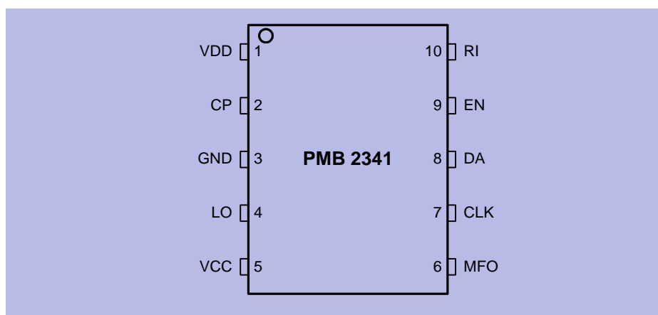
Figure 3-1 IC Pin Configuration
