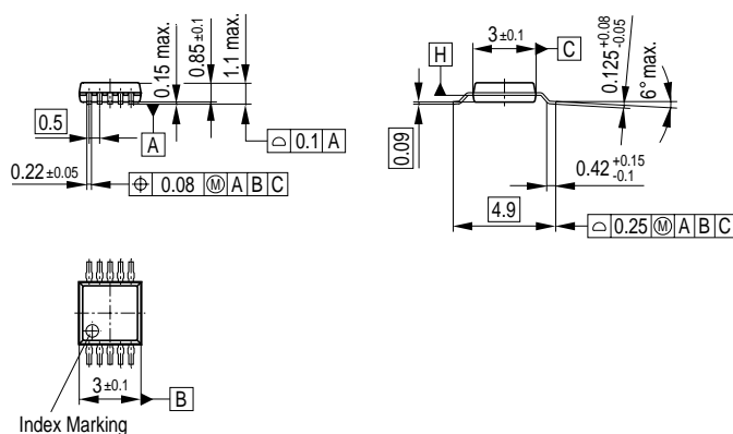
Figure 2-1 Mini-TSSOP-10
