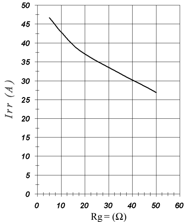
Fig. 18 – Typical Diode I_{RR} vs. R_g I_F = 50\text{A} ; T_j = 125^\circ\text{C}
