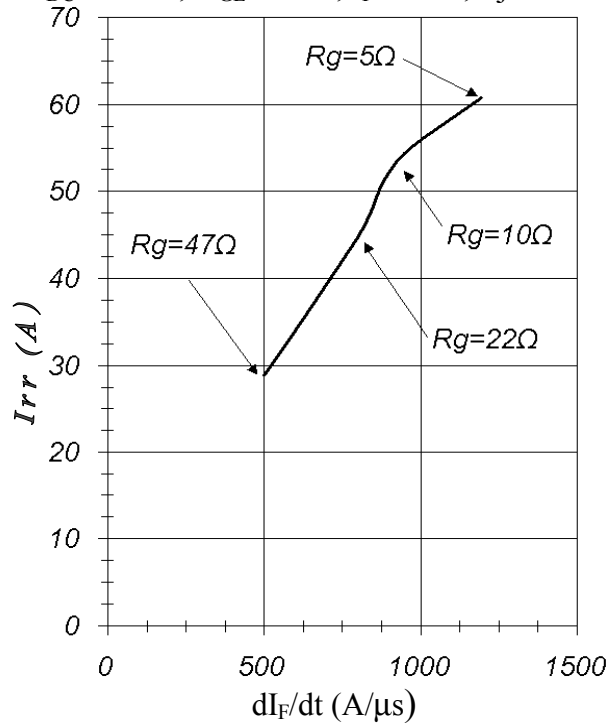
Fig. 19 – Typical Diode I_{RR} vs. dI_F/dt V_{DC} = 600\text{V} ; V_{GE} = 15\text{V} ; I_F = 25\text{A} ; T_j = 125^\circ\text{C}
