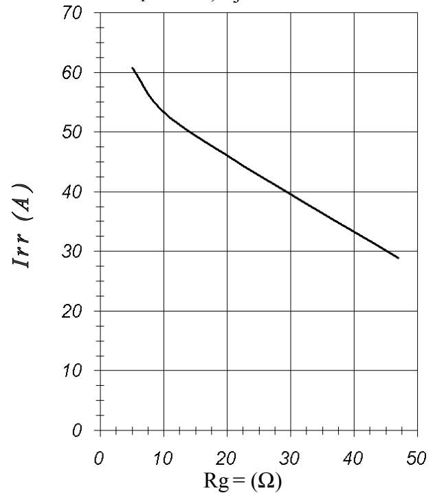
Fig. 18 – Typical Diode I_{RR} vs. R_g I_F = 25\text{A} ; T_j = 125^\circ\text{C}
