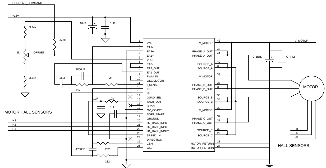
Fig 5: Implementation of a Current-Mode Controller
