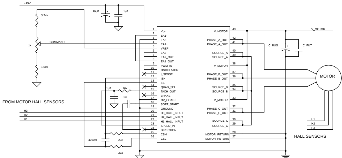
Fig 4: Implementation of a Voltage-Mode Controller
