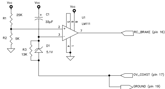
Fig 3: Optional Start-Up Circuit
