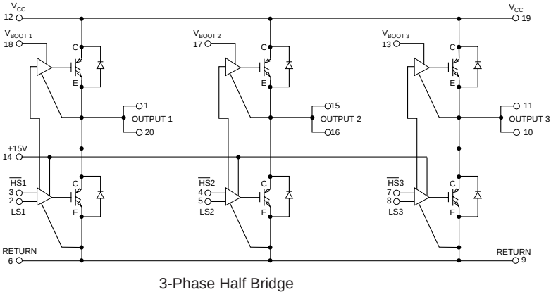
3-Phase Half Bridge
