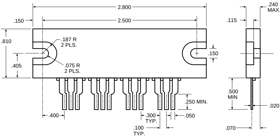
Omnirel Package P-2 (Industrial 12-Pin)
