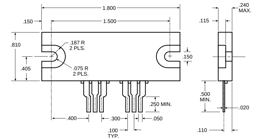
Omnirel Package P-2 (Industrial 12-Pin)
