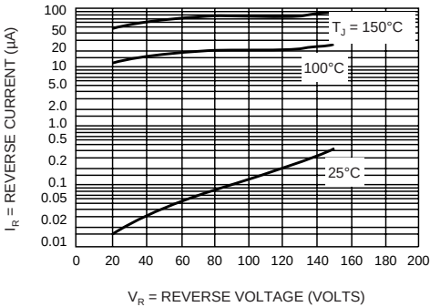
TYPICAL REVERSE CURRENT OM5236, 5237, 5238, 5239
