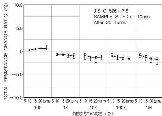
Fig.6-1 Endurance (wiper)
