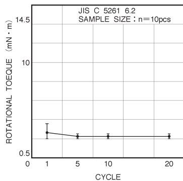
Fig. 7 Rotational torque
