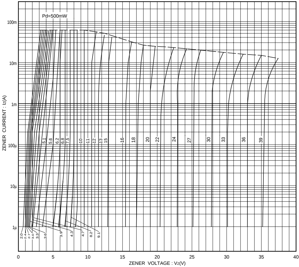
Fig. 1 Zener characteristics
