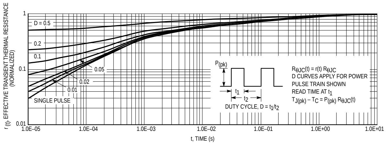
Figure 13. Thermal Response
