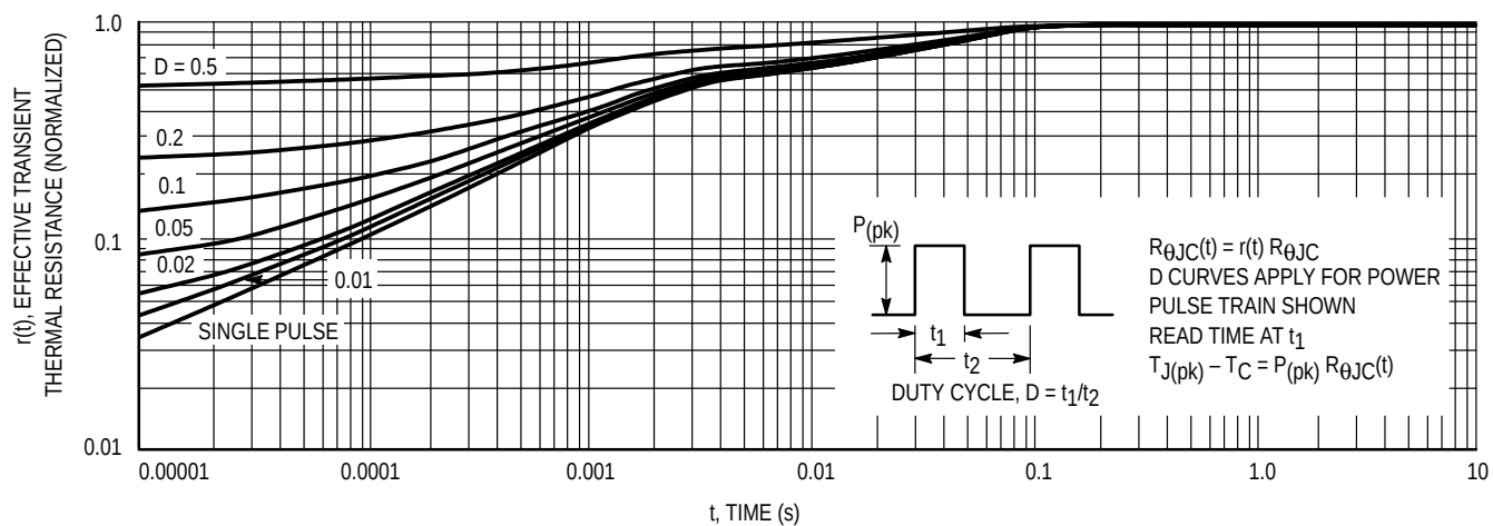
Figure 14. Thermal Response
