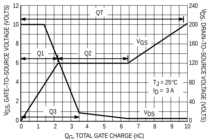
Figure 8. Gate-To-Source and Drain-To-Source Voltage versus Ttotal Charge
