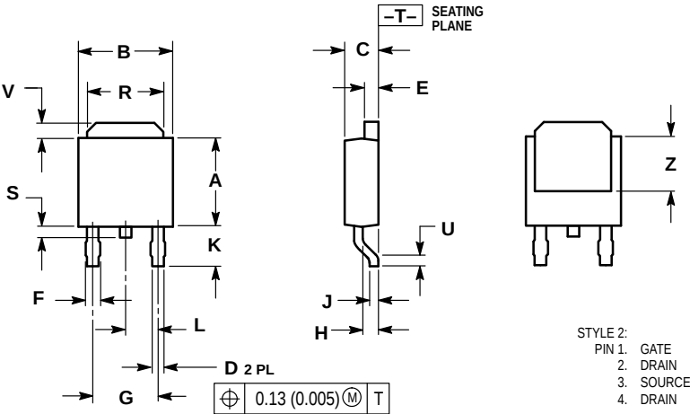
CASE 369A-13 ISSUE W
