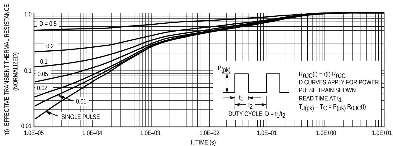
Figure 14. Thermal Response
