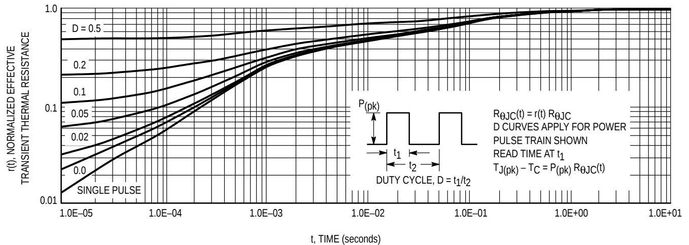
Figure 13. Thermal Response
