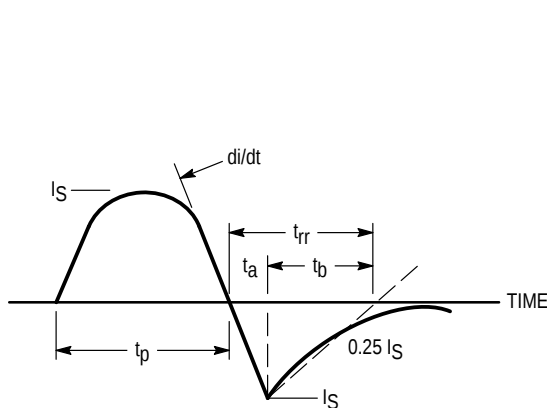
Figure 14. Diode Reverse Recovery Waveform
