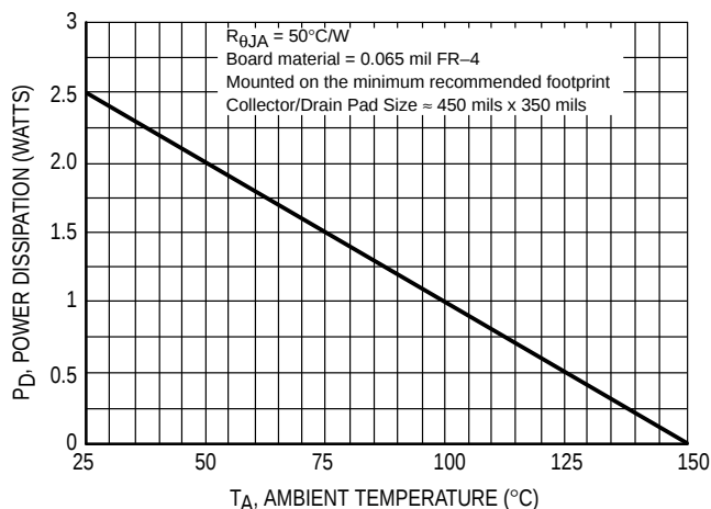
Figure 13. D 2 PAK Power Derating Curve
