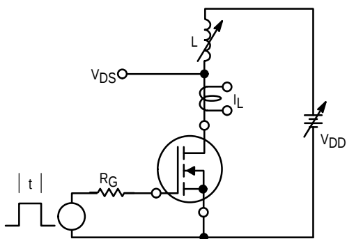
Figure 11. Unclamped Inductive Switching Test Circuit
