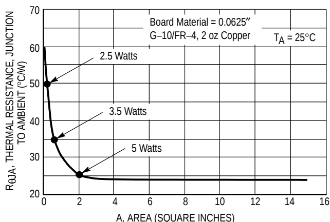
Figure 15. Thermal Resistance versus Drain Pad Area for the D 2 PAK Package (Typical)
