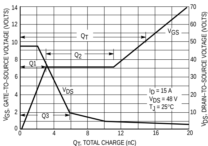
Figure 6. Gate-to-Source and Drain-to-Source Voltage versus Total Charge
