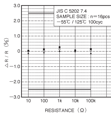
Fig.10 Temperature cycling
