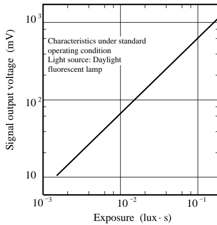
Photoelectric Conversion Characteristics
