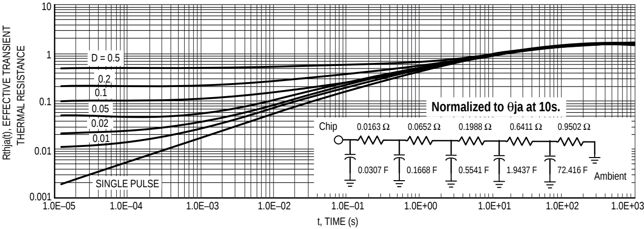
Figure 14. Thermal Response
