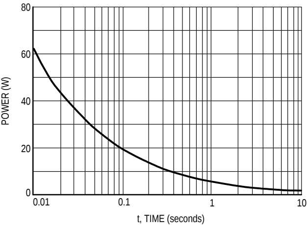
Figure 17. Single Pulse Power
