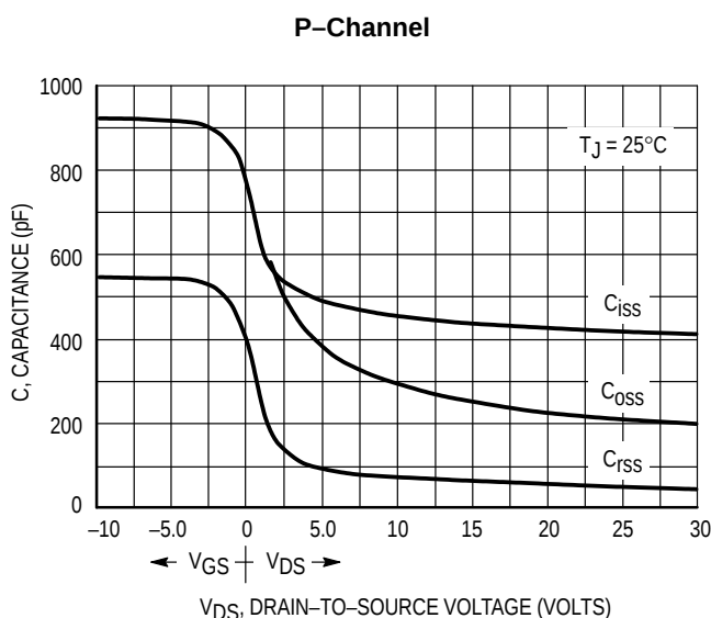
Figure 7. Capacitance Variation
