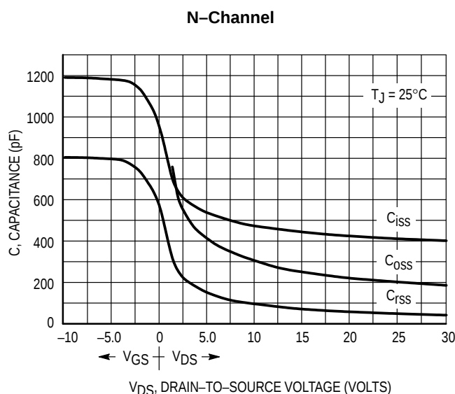
Figure 7. Capacitance Variation
