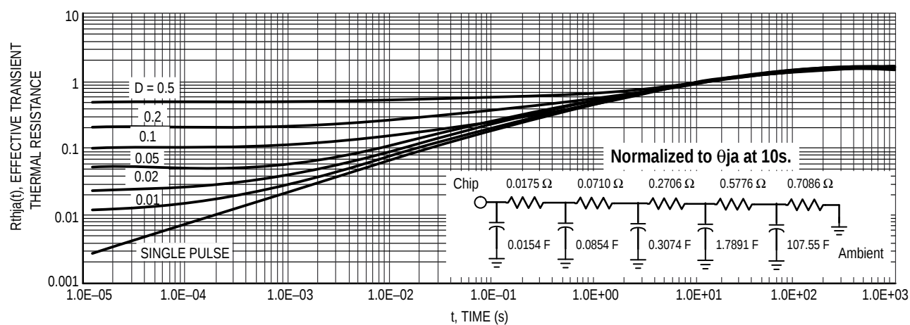
Figure 14. Thermal Response
