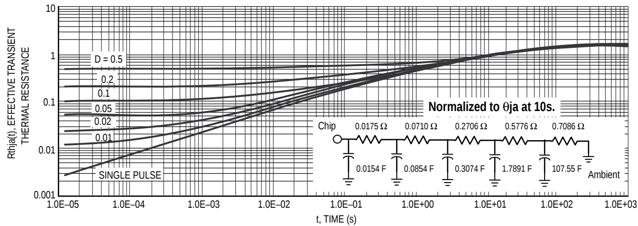
Figure 10. Thermal Response
