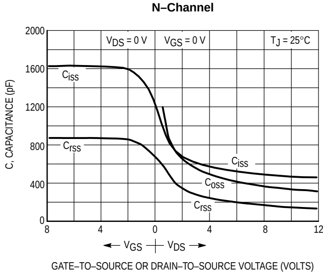
Figure 7. Capacitance Variation
