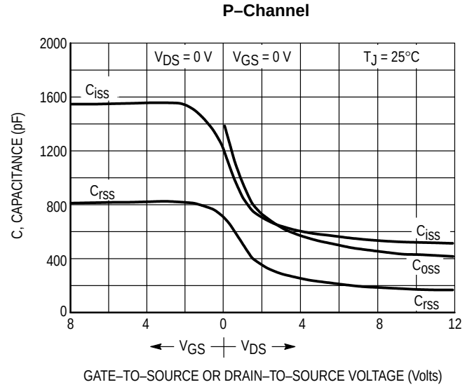
Figure 7. Capacitance Variation
