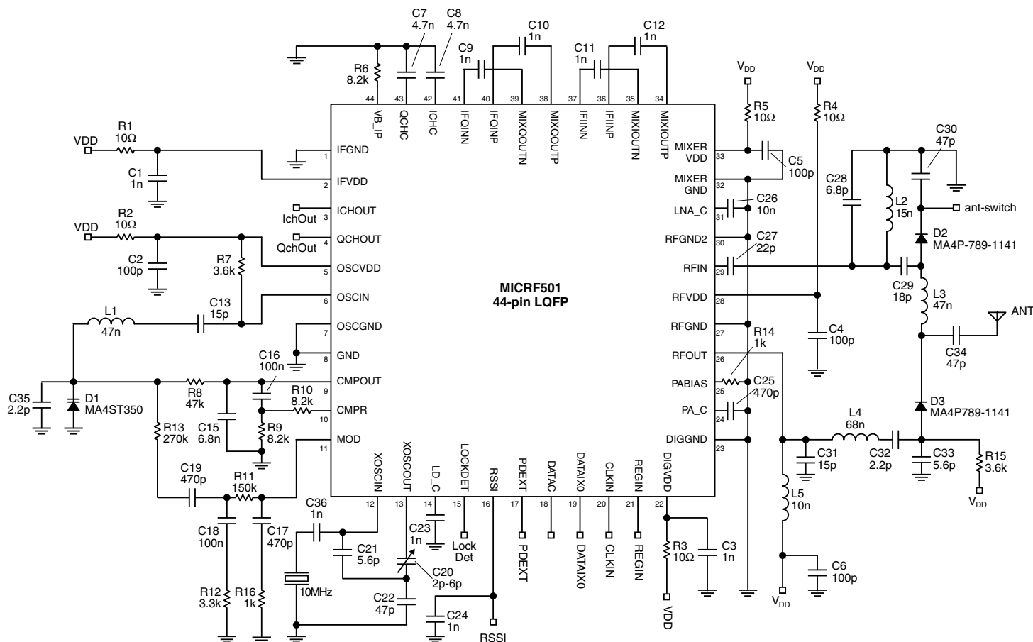
Figure 3. Application Circuit
