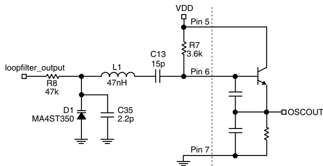
Figure 3. VCO
