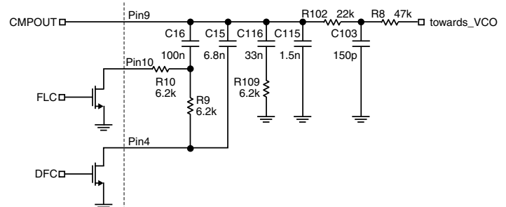
Figure 7. Dual-Loop Filters
