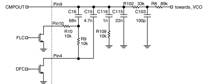
Figure 7. Dual-Loop Filters
