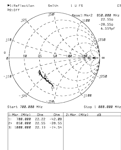
Figure 8. Input Impedance
