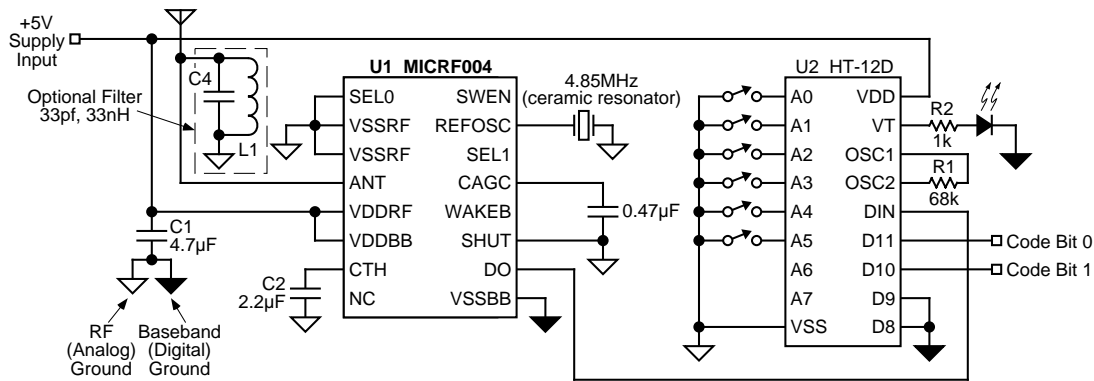
Figure 7a. 150MHz, 1kb/s On-Off Keyed Receiver/Decoder
