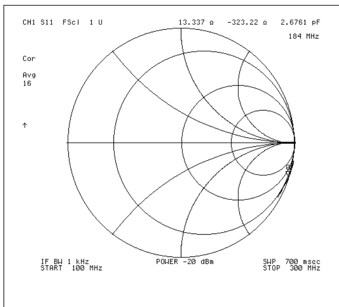
Antenna Impedance
