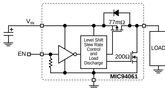
Load Switch Application with Capacitive Load Discharge
