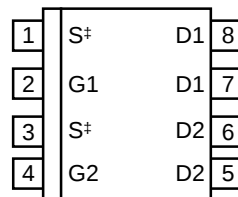
8-lead Low-Profile SOIC Package (LM)
