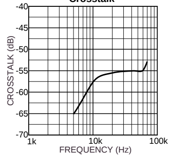
Channel-to-Channel Crosstalk
