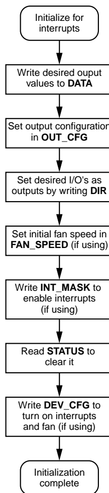
Figure9b. Initializing the MIC74 for Interrupts
