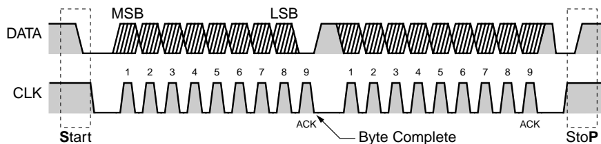
Figure 5. Serial Byte Format
