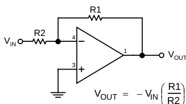
Figure 2. Inverting Amplifier
