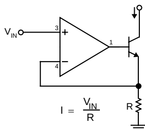
Figure 3. Voltage Controlled Current Sink
