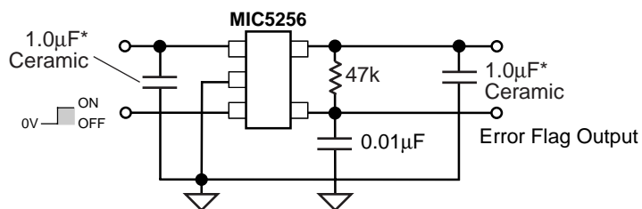
Figure 1. Test Circuit
