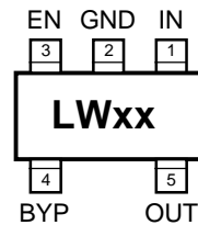
MIC5255-x.xBM5 (SOT-23-5)
