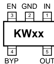
MIC5255-x.xYM5 (SOT-23-5)
