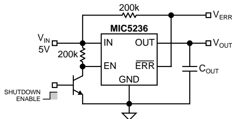
Figure 1. Remote Enable
