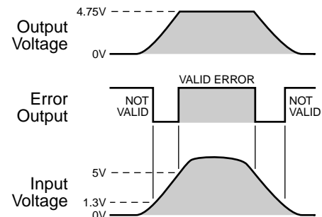
Figure 3. Error Output Timing
