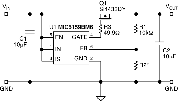
Application Circuit
