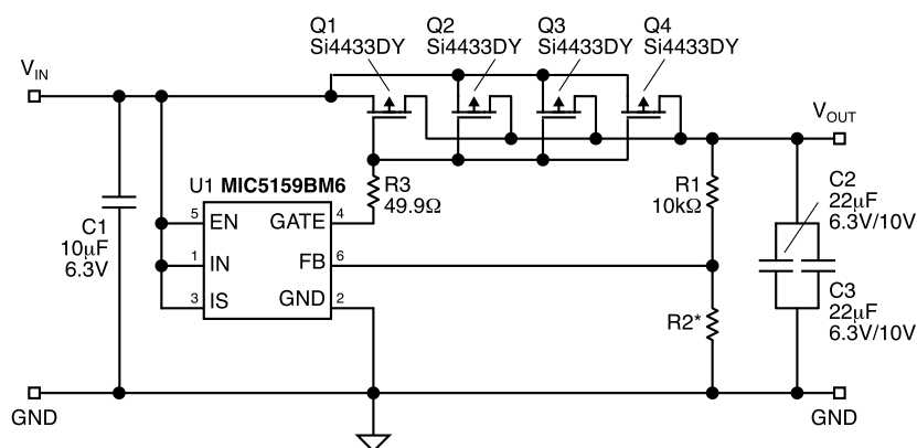
Application Circuit
