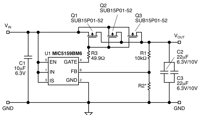
Application Circuit
