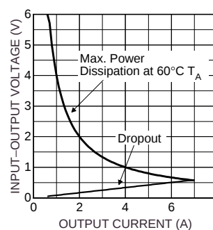
Si4433DY x4 SOA
