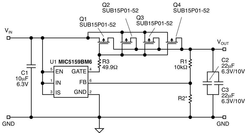
Application Circuit
