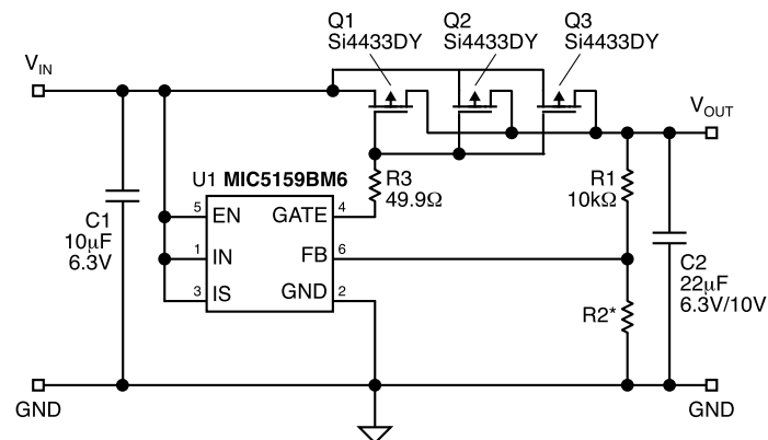
Application Circuit
