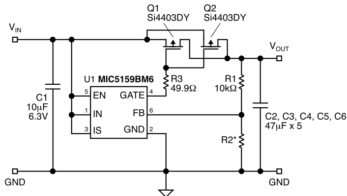
Application Circuit
