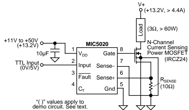
Figure 3. Using a Current Sensing MOSFET
