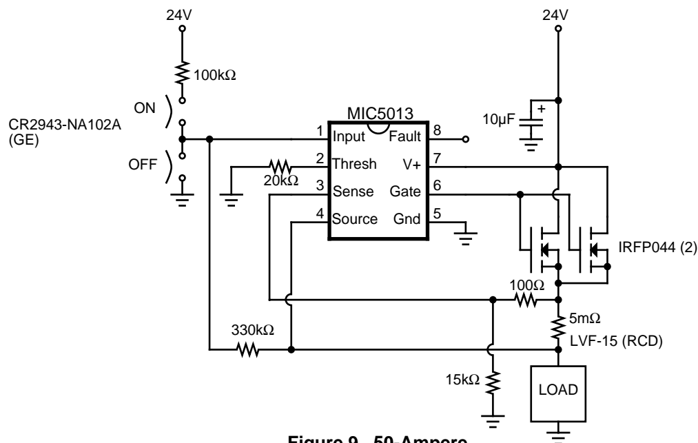
Figure 9. 50-Ampere Industrial Switch
