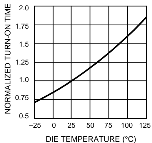
Turn-on Time
