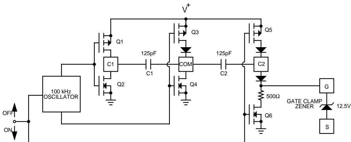
Figure 12. Gate Control Circuit Detail
