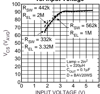
CS Voltage vs. Input Voltage
