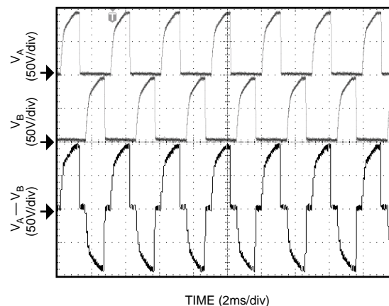
Figure 4. 360Hz Output Waveform
