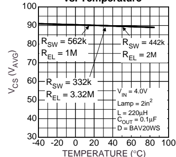
CS Voltage vs. Temperature
