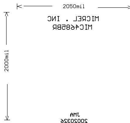
Figure 5b. Bottom Silk Screen
