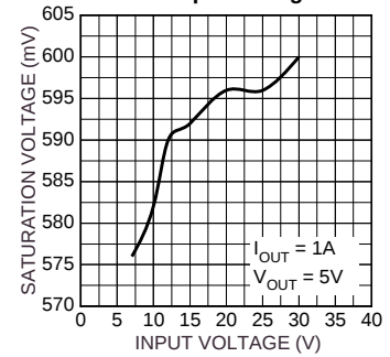
Saturation Voltage vs. Input Voltage
