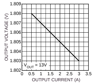
Load Regulation
