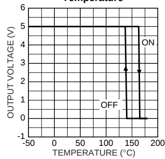
Shutdown Hysteresis vs. Temperature
