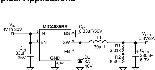
1.8V Output Converter
