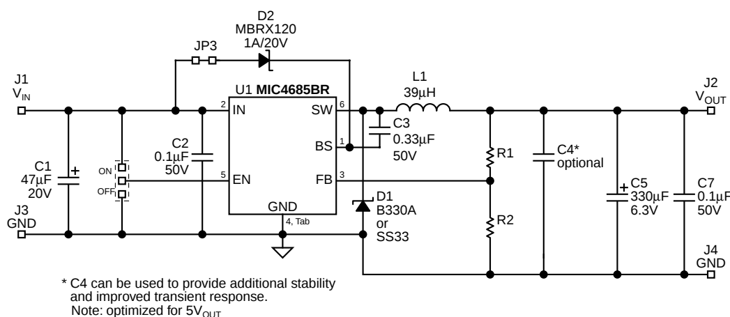
Figure 3. Schematic Diagram
