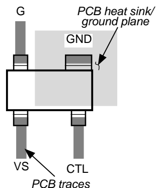
Figure 4. Heat-Sink Plane
