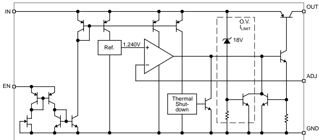
MIC3975 Adjustable Regulator Block Diagram
