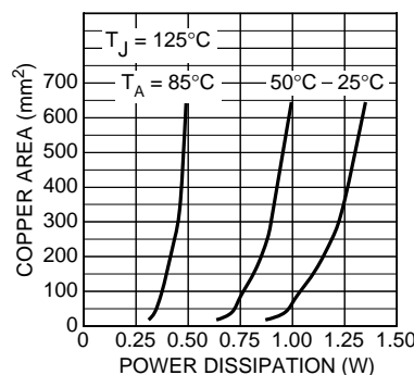
Figure 5. Copper Area vs. Power-SOP Power Dissipation
