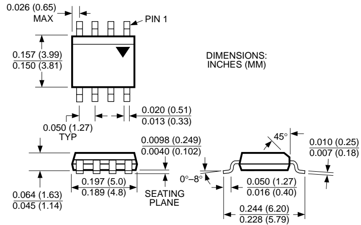
SOP-8 (M)
